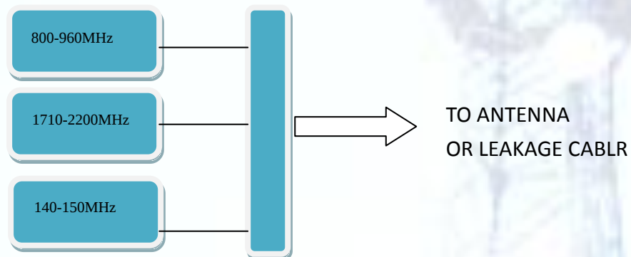
3 BAND COMBINER
